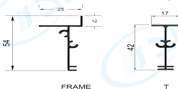
FRAME
